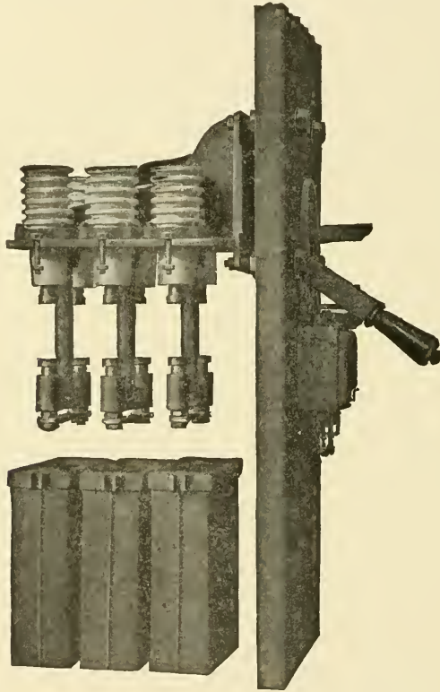
Fig. 155. Hand-Operated Automatic, 300-Ampere, 3-Pole Circuit Breaker. Open Position
